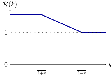
FIGURE 4.—The ratio of gross to net exposures as a function of k , in the three-types model.
