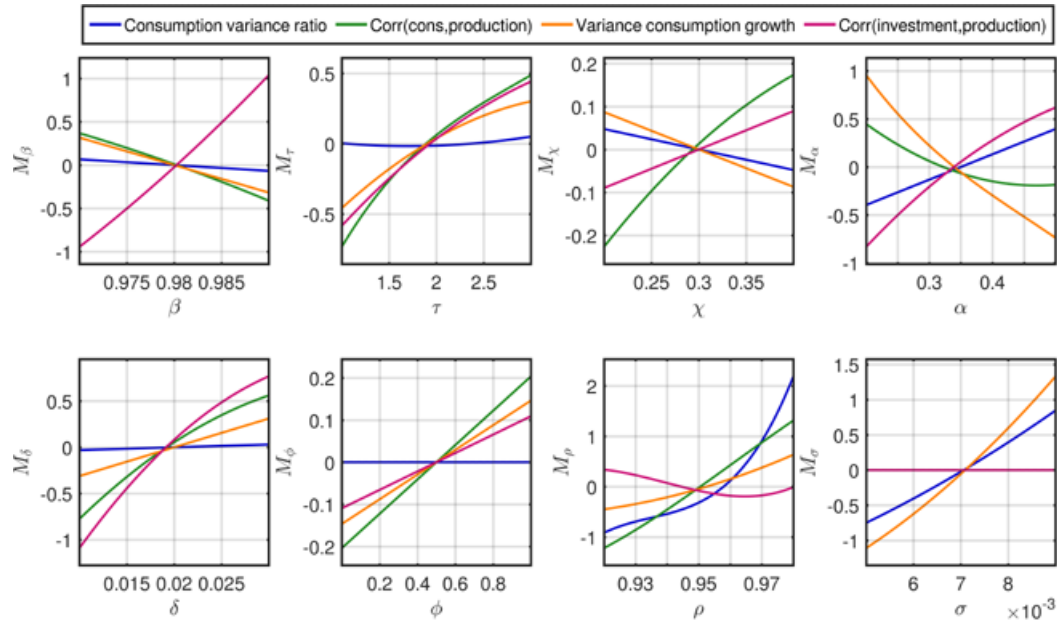
FIGURE 11. Univariate effects.
