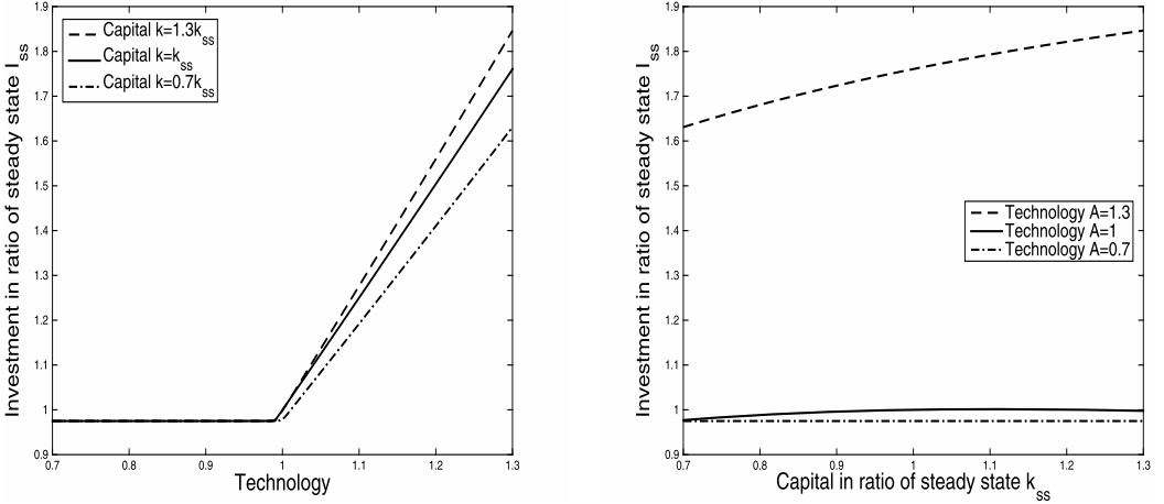
FIGURE 6. Investment policy function for the RBC model with a constraint on investment.
