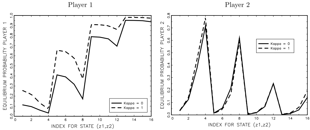
FIGURE 3. Equilibrium probabilities.
