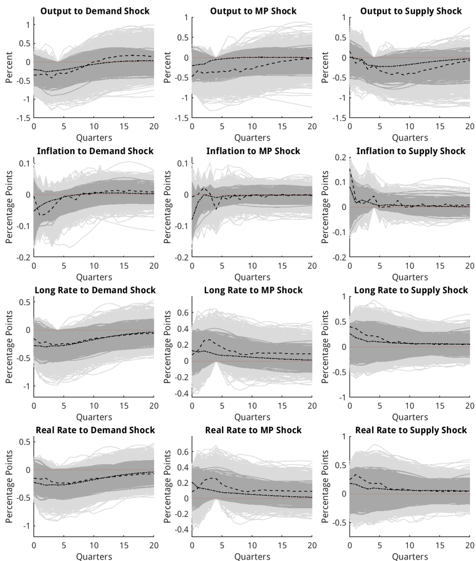
FIGURE 5.—Bayes estimator of joint posterior impulse responses (dashed black lines) and its 68 percent credible set under the additively separable absolute loss function under uniform joint prior distribution for the vector of impulse responses (solid light gray lines) and under the Minnesota prior (dashed-dotted lines and solid dark gray lines for the 68 percent credible set).
