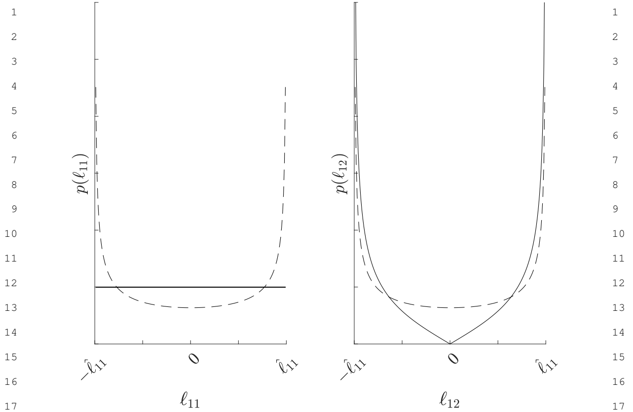
FIGURE 2.—The dotted lines are the conditional densities of \ell_{11} and \ell_{12} for Case (1). The solid lines are the conditional densities of \ell_{11} and \ell_{12} for Case (2).
