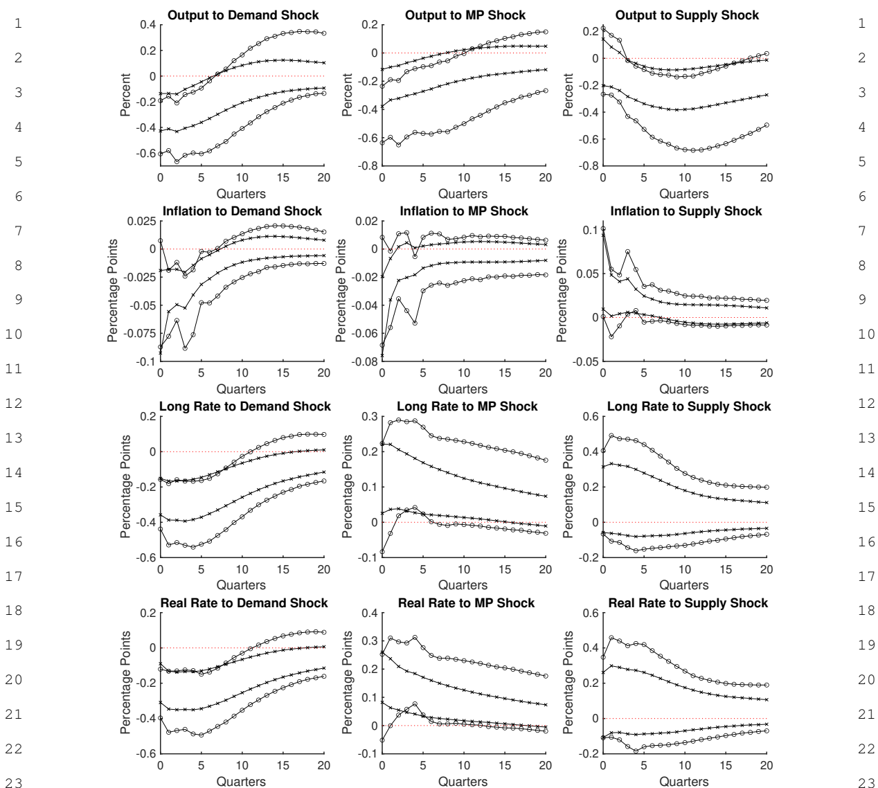
FIGURE 3.—The solid lines with circle (o) markers depict the equal-tailed 68 percent marginal posterior probability bands of individual impulse responses implied by the uniform joint prior distribution for the vector of impulse responses. The solid lines with cross (x) markers depict the equal-tailed 68 percent marginal posterior probability bands of individual impulse responses implied by the Minnesota prior.
