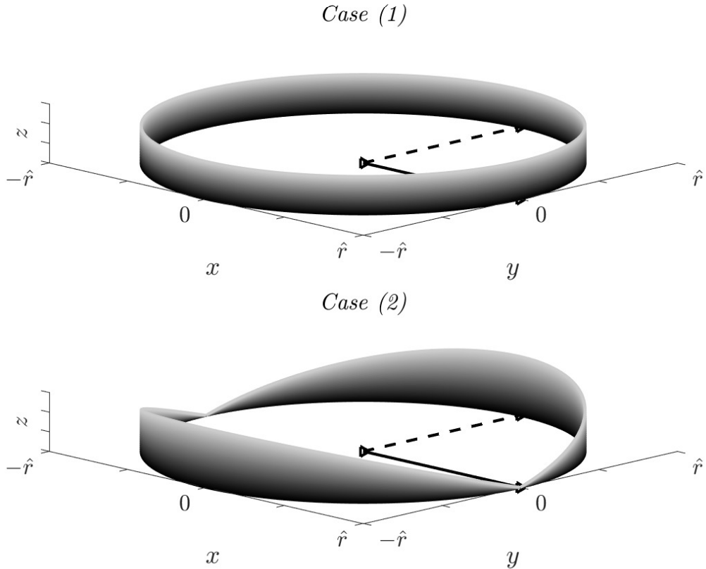
FIGURE 1.—Conditional joint density for Cases (1) and (2). The solid vector is \hat{\mathbf{L}}_{\cos}^i \in \mathbb{R}^4 , the dotted vector is \hat{\mathbf{L}}_{\sin}^i \in \mathbb{R}^4 , and z = p(\mathbf{L}_0) , with \mathbf{L}_0 = (x\hat{\mathbf{L}}_{\cos}^i + y\hat{\mathbf{L}}_{\sin}^i)/\hat{r} .
