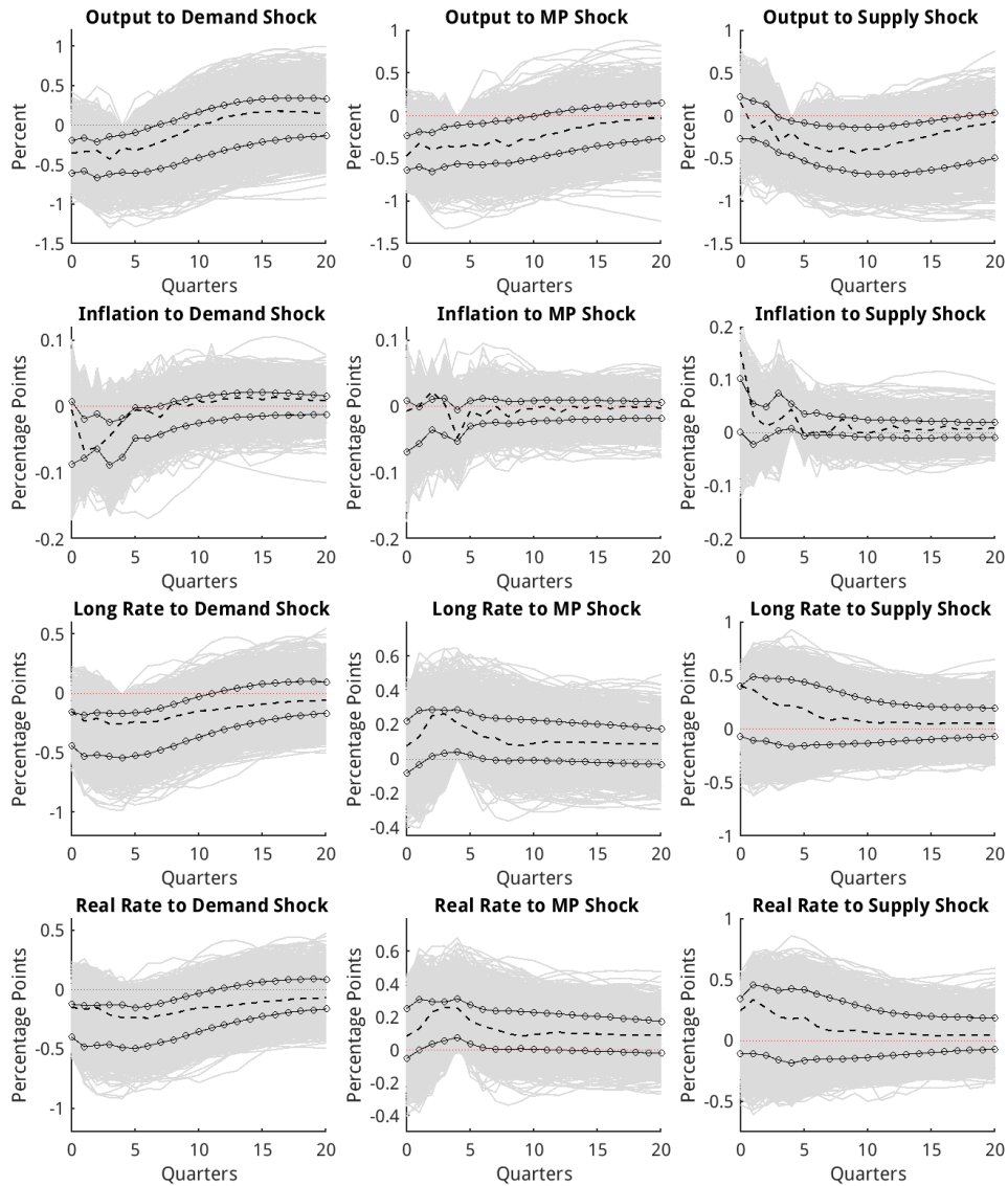
FIGURE 4.—Bayes estimator of the joint posterior distribution for the vector of impulse responses (dashed lines) and its 68 percent credible set (solid light gray lines) under the additively separable absolute loss function. The solid lines with circle (o) markers depict the equal-tailed 68 percent unconditional prior distributions for individual impulse responses. Both posteriors are implied by the uniform joint prior distribution for the vector of impulse responses.
