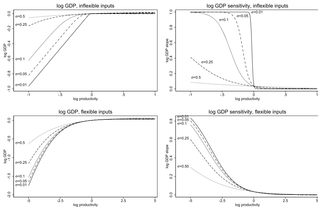
FIGURE 3.—Numerical examples. Notes: The panels report the effect of shocking log productivity in a single sector, holding all others fixed. The right-hand panels report the local response of log GDP to the sector’s productivity (its Domar weight).
