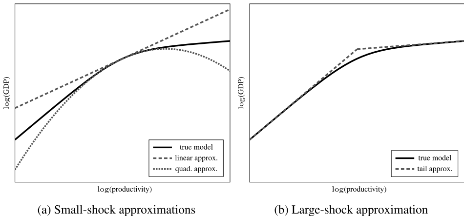
FIGURE 2. —Linear, quadratic, and tail approximations. Notes: The x-axis is log productivity and the y-axis log aggregate output. The x-axis may represent productivity in a single sector, or it could be the scale of a shock that affects productivity in multiple sectors. The concavity in GDP in this example is consistent with an economy featuring complementarities.
