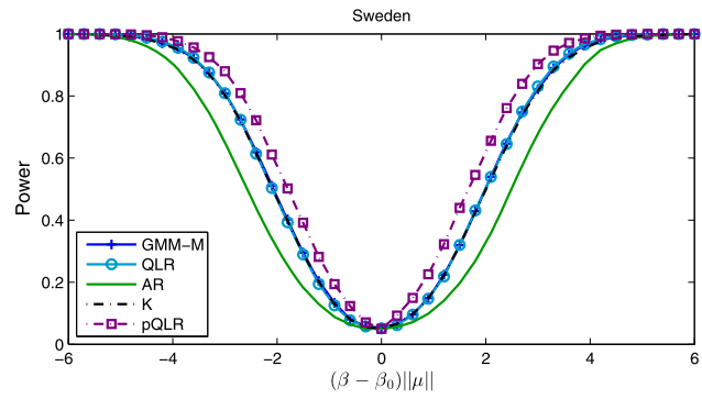
FIGURE S2.—Power functions for the GMM-M, QLR, AR (or S ), K , and pQLR tests in simulation calibrated to Yogo (2004) data.
