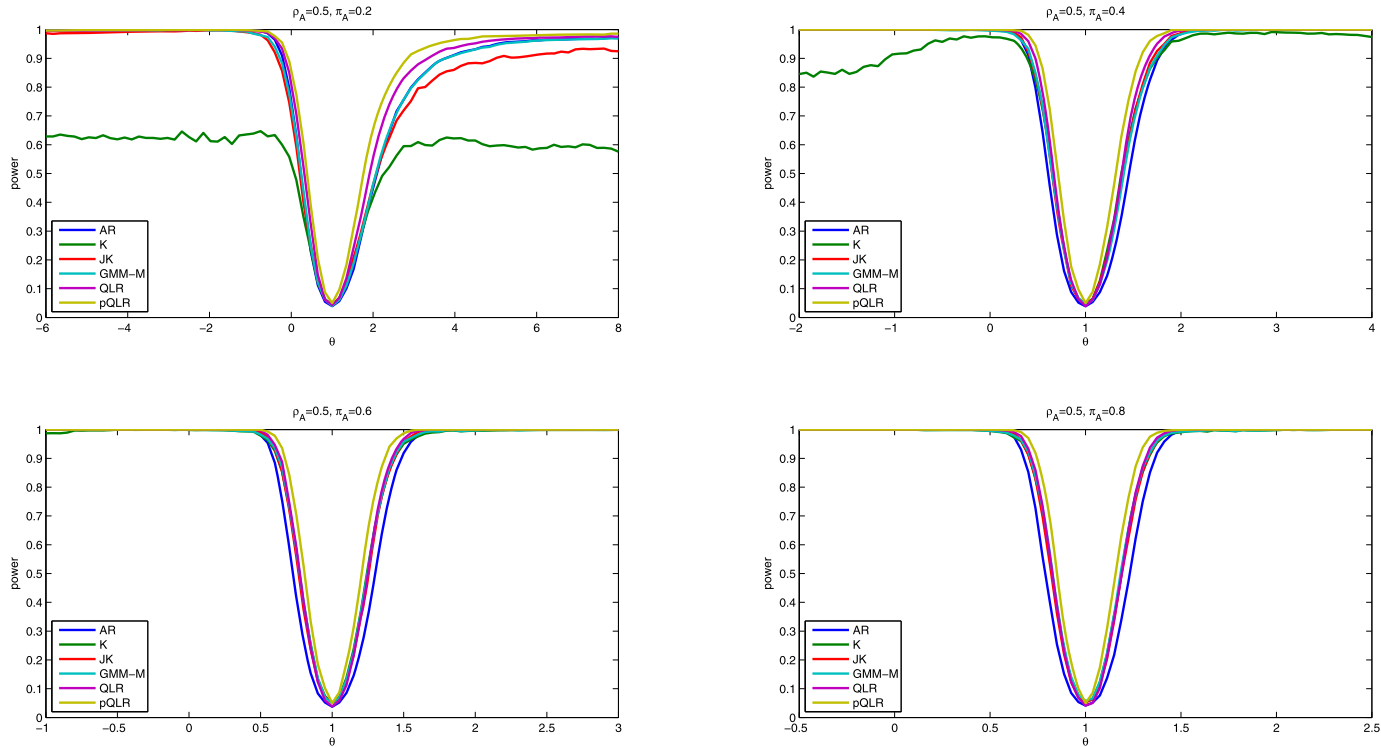
FIGURE S14.—Simulated power of nominal 5% tests in asymmetric quantile IV simulation design with \rho_A = 0.5 , 5 instruments, and 1,000 observations. Based on 2,500 simulation replications and 1,000 draws of conditional critical values.
