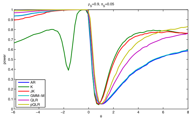
FIGURE S6.—Simulated power of nominal 5% tests in symmetric quantile IV simulation design with \rho_S = 0.9 , 10 instruments, and 1,000 observations. Based on 2,500 simulation replications and 1,000 draws of conditional critical values.
