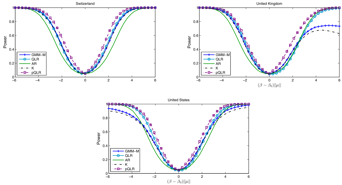
FIGURE S3.—Power functions for the GMM-M, QLR, AR (or S ), K , and pQLR tests in simulation calibrated to Yogo (2004) data.
