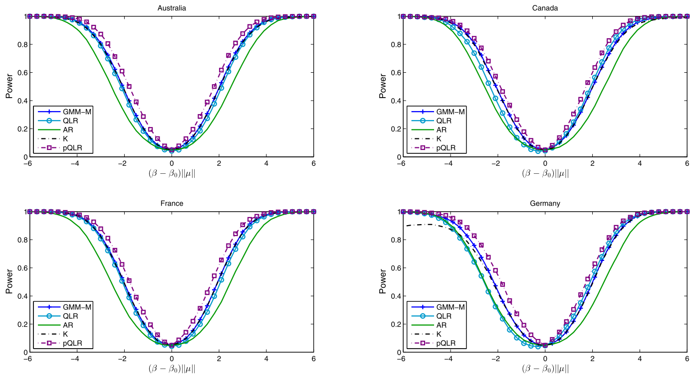
FIGURE S1.—Power functions for the GMM-M, QLR, AR (or S ), K , and pQLR tests in simulation calibrated to Yogo (2004) data.
