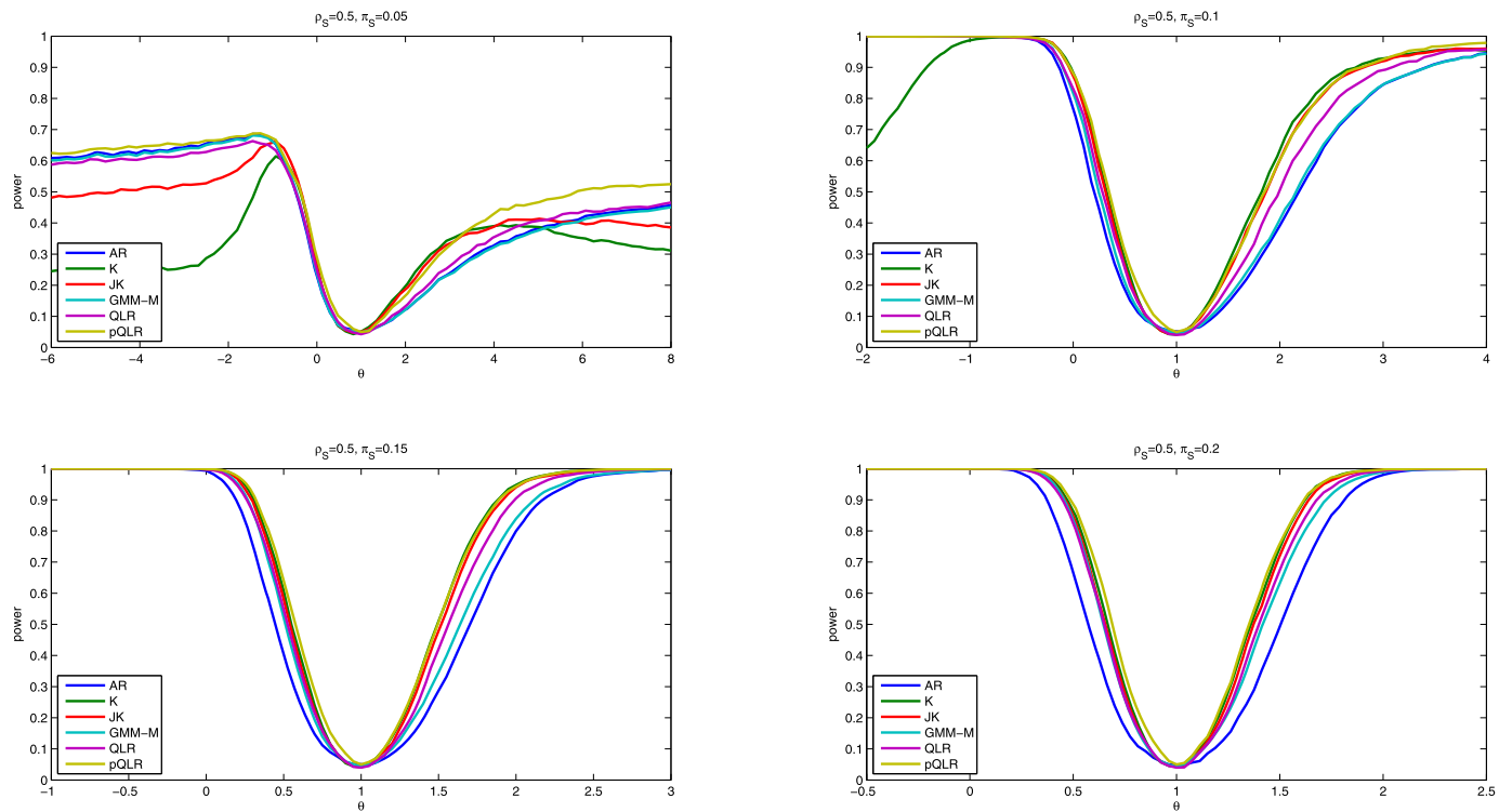
FIGURE S11.—Simulated power of nominal 5% tests in symmetric quantile IV simulation design with \rho_S = 0.5 , 5 instruments, and 1,000 observations. Based on 2,500 simulation replications and 1,000 draws of conditional critical values.
