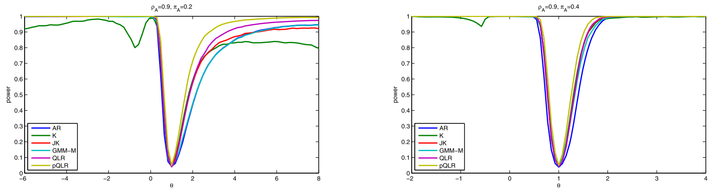
FIGURE S15.—Simulated power of nominal 5% tests in asymmetric quantile IV simulation design with \rho_A = 0.9 , 5 instruments, and 1,000 observations. Based on 2,500 simulation replications and 1,000 draws of conditional critical values.
