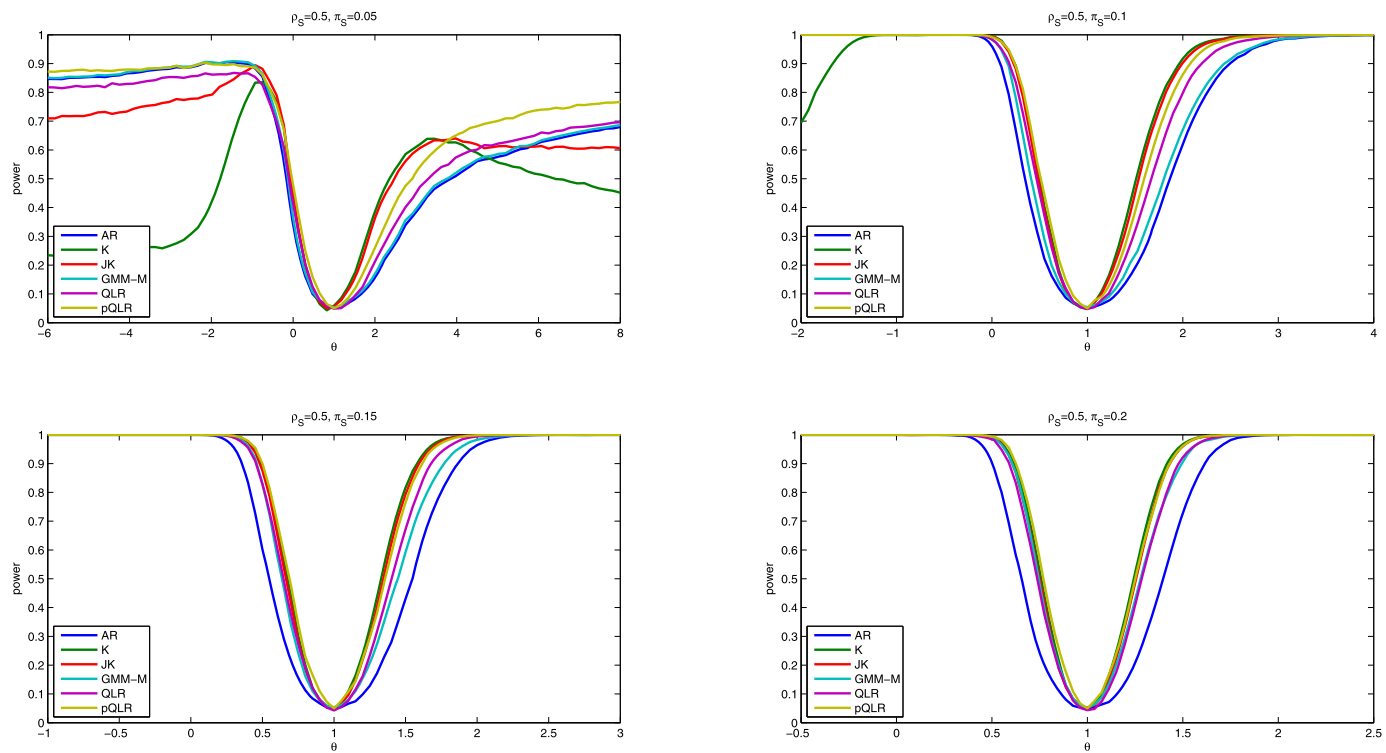
FIGURE S5.—Simulated power of nominal 5% tests in symmetric quantile IV simulation design with \rho_S = 0.5 , 10 instruments, and 1,000 observations. Based on 2,500 simulation replications and 1,000 draws of conditional critical values.
