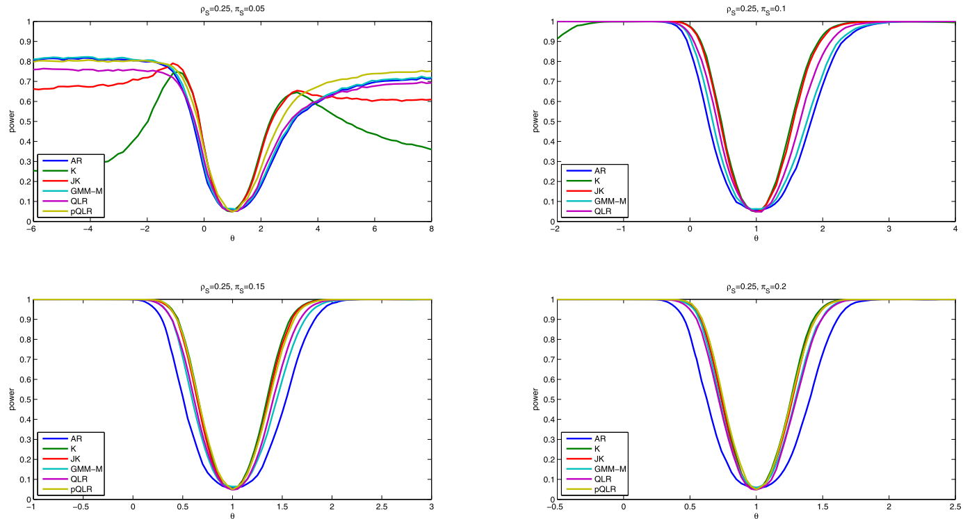
FIGURE S4.—Simulated power of nominal 5% tests in symmetric quantile IV simulation design with \rho_S = 0.25 , 10 instruments, and 1,000 observations. Based on 2,500 simulation replications and 1,000 draws of conditional critical values.
