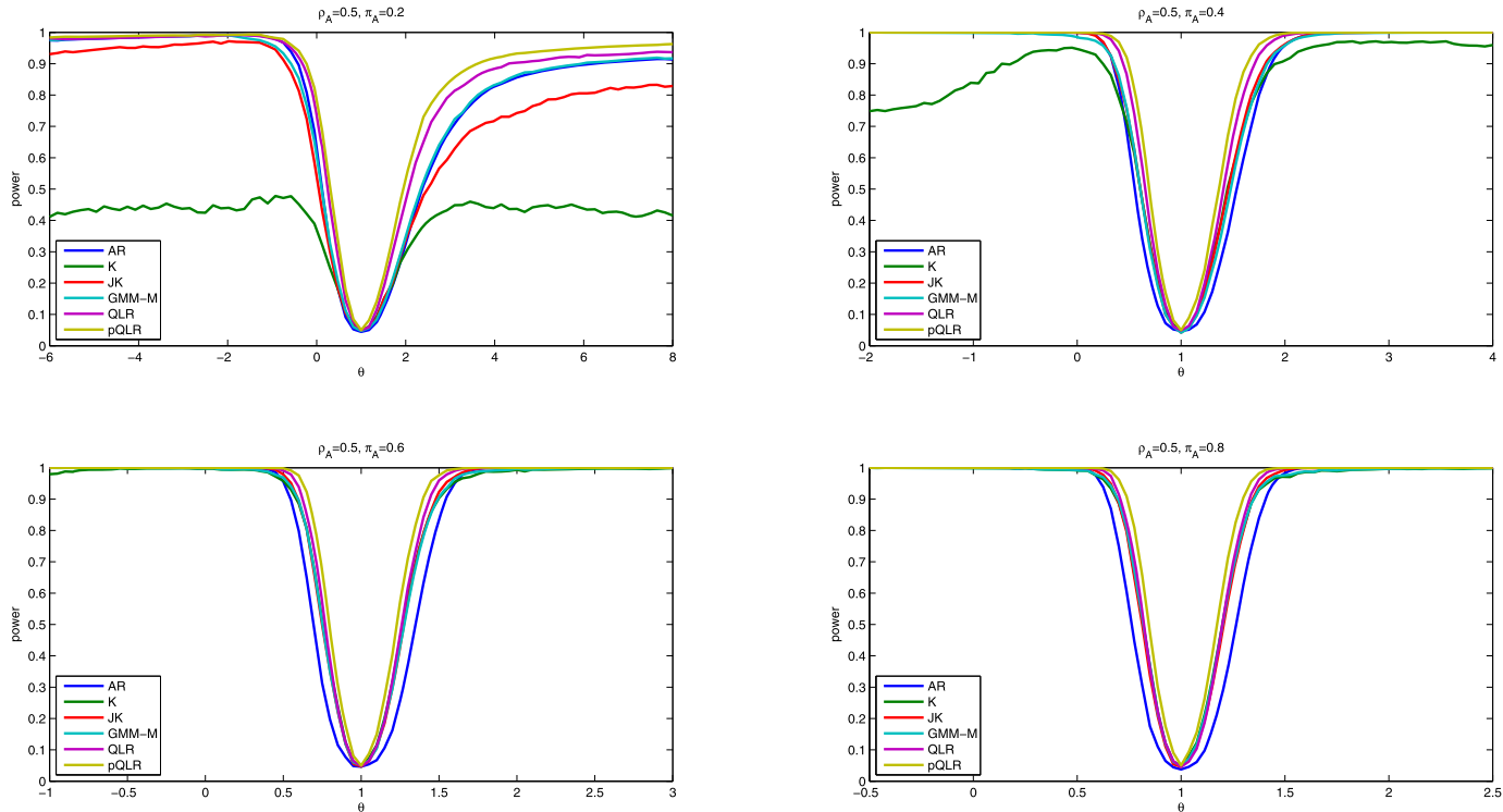
FIGURE S8.—Simulated power of nominal 5% tests in asymmetric quantile IV simulation design with \rho_A = 0.5 , 10 instruments, and 1,000 observations. Based on 2,500 simulation replications and 1,000 draws of conditional critical values.
