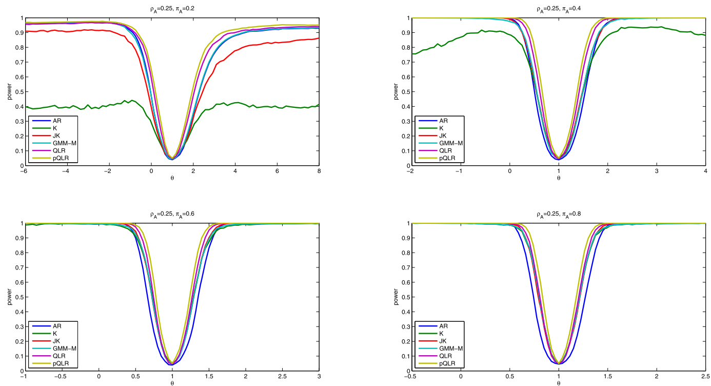
FIGURE S7.—Simulated power of nominal 5% tests in asymmetric quantile IV simulation design with \rho_A = 0.25 , 10 instruments, and 1,000 observations. Based on 2,500 simulation replications and 1,000 draws of conditional critical values.
