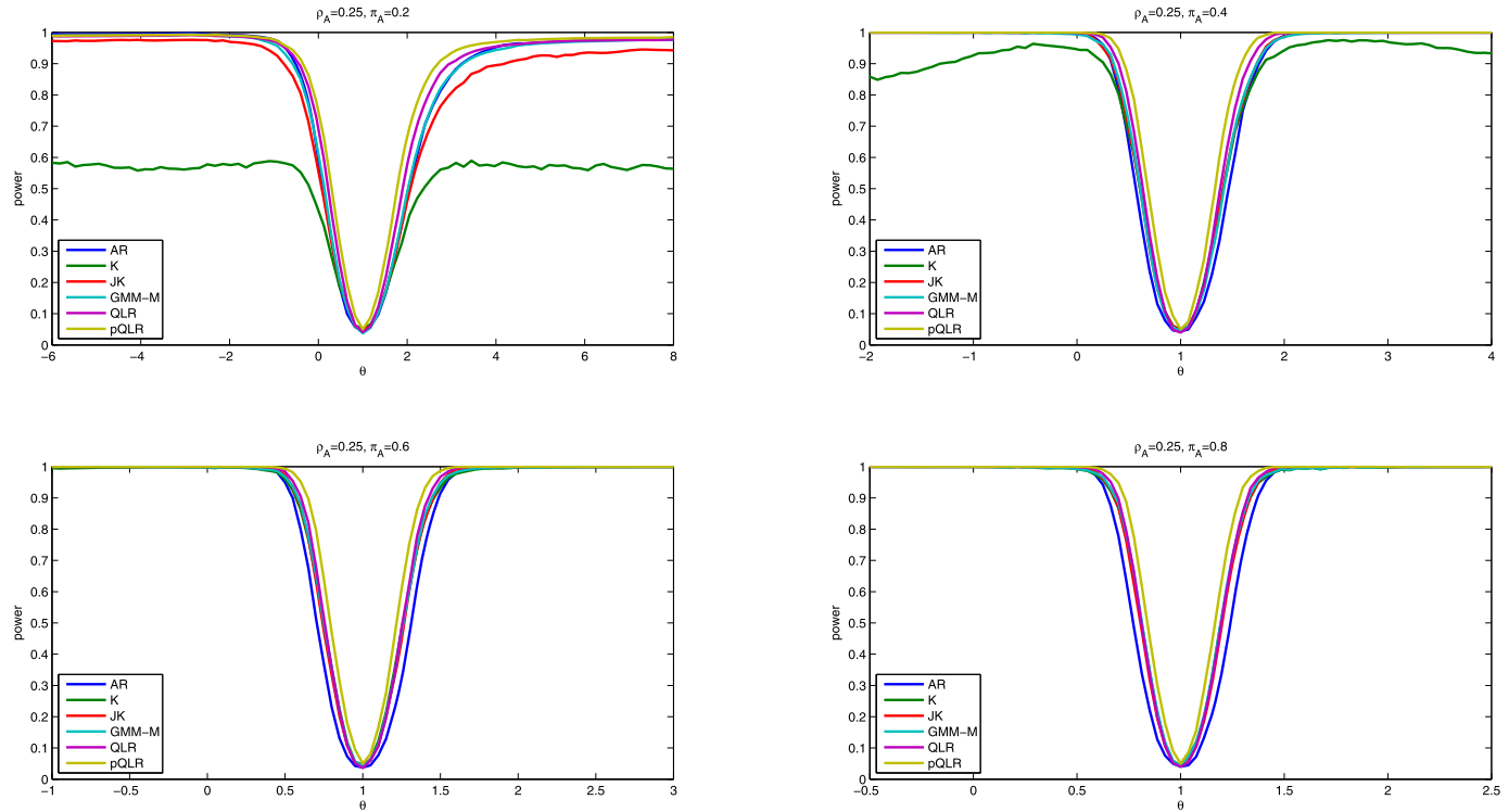
FIGURE S13.—Simulated power of nominal 5% tests in asymmetric quantile IV simulation design with \rho_A = 0.25 , 5 instruments, and 1,000 observations. Based on 2,500 simulation replications and 1,000 draws of conditional critical values.
