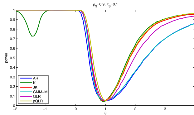
FIGURE S12.—Simulated power of nominal 5% tests in symmetric quantile IV simulation design with \rho_S = 0.9 , 5 instruments, and 1,000 observations. Based on 2,500 simulation replications and 1,000 draws of conditional critical values.
