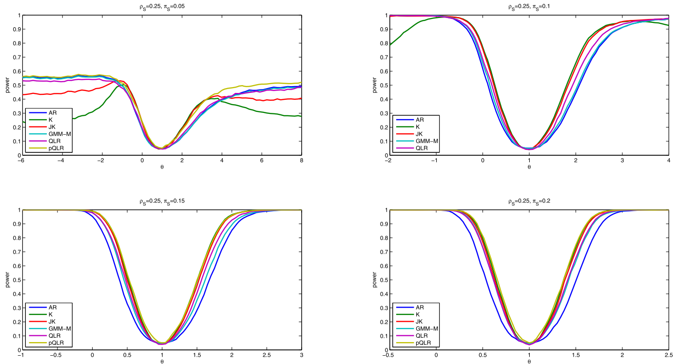
FIGURE S10.—Simulated power of nominal 5% tests in symmetric quantile IV simulation design with \rho_S = 0.25 , 5 instruments, and 1,000 observations. Based on 2,500 simulation replications and 1,000 draws of conditional critical values.
