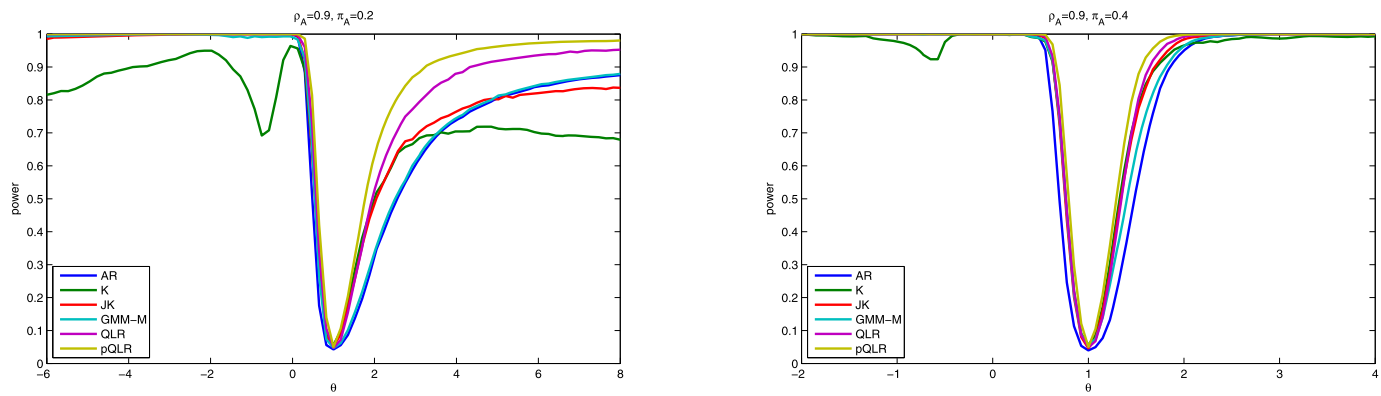
FIGURE S9.—Simulated power of nominal 5% tests in asymmetric quantile IV simulation design with \rho_A = 0.9 , 10 instruments and 1,000 observations. Based on 2,500 simulation replications and 1,000 draws of conditional critical values.
