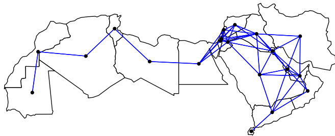
Figure 16: Inverse distance matrix ( W_{dinverse} )
