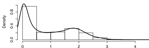
Estimated beta
