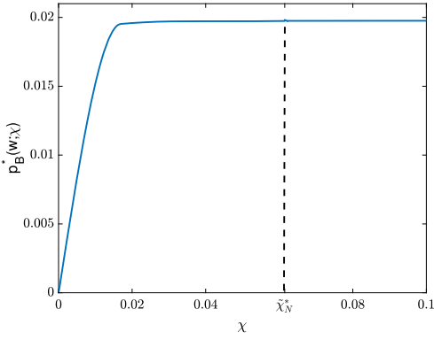
(a) p_B^*(\chi)
