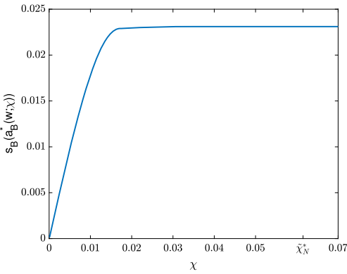
(c) s_B(\chi)
