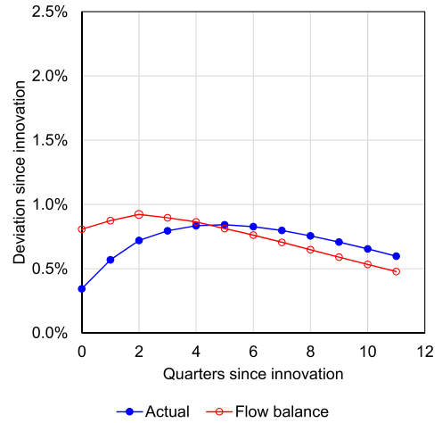
FIGURE 11. Descriptive impulse responses: model extensions.
