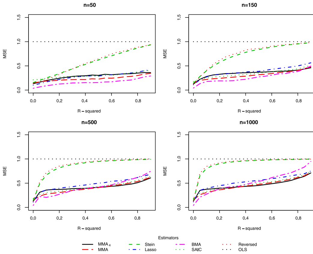
FIGURE 15. Model 4: \alpha = 2 .
