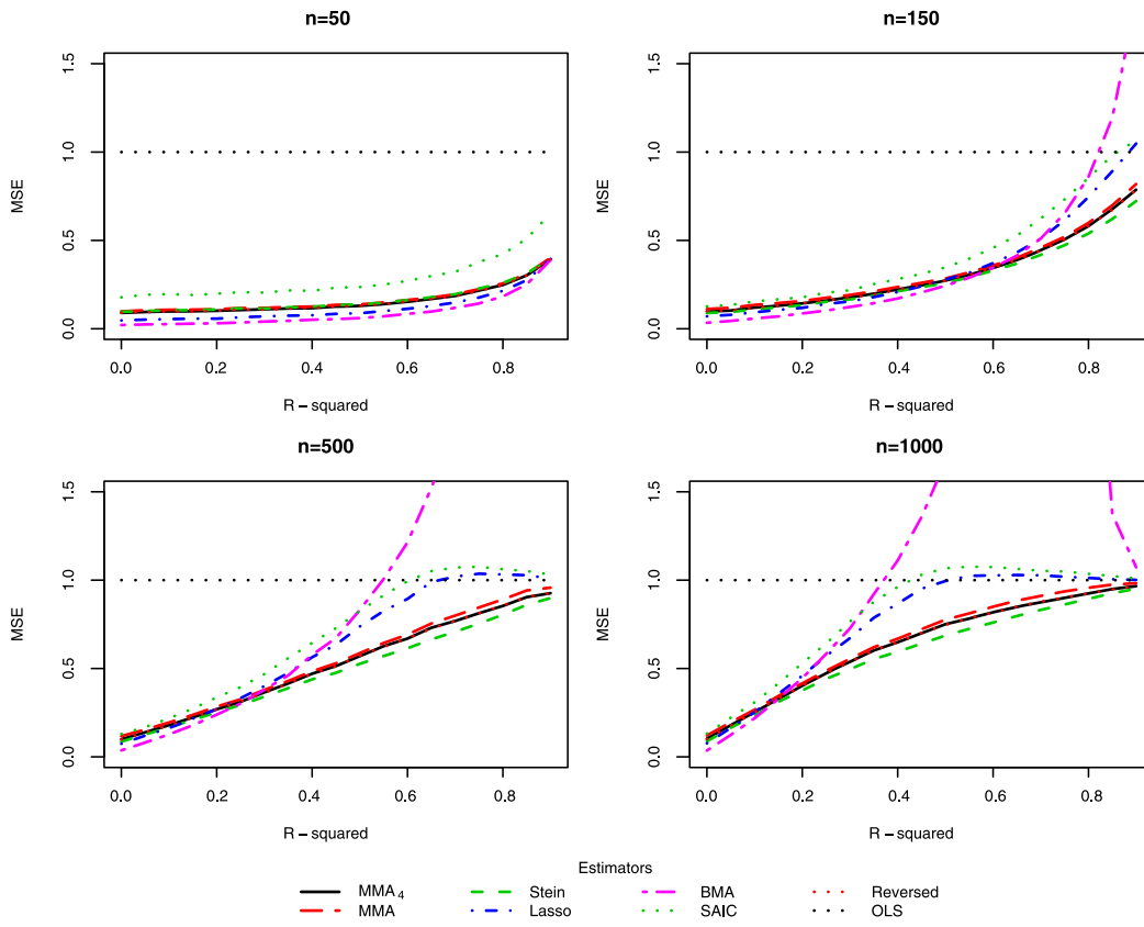
FIGURE 17. Model 5: \alpha = 0 .
