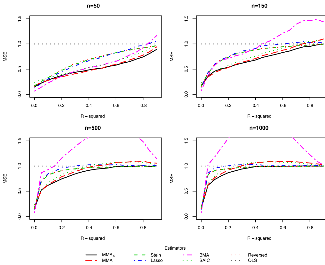
FIGURE 6. Model 2: \alpha = 1 .
