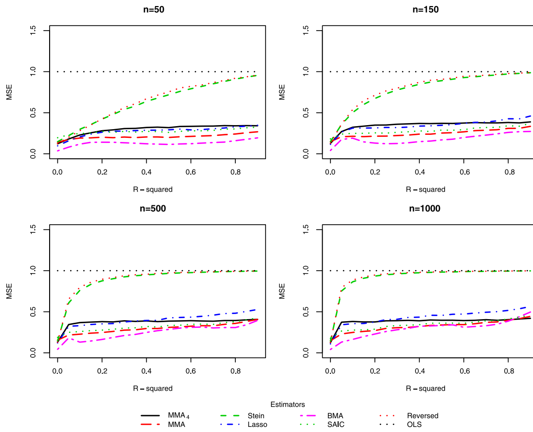
FIGURE 16. Model 4: \alpha = 3 .
