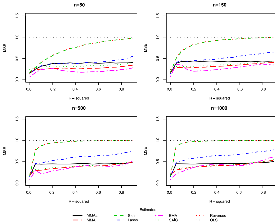
FIGURE 8. Model 2: \alpha = 3 .
