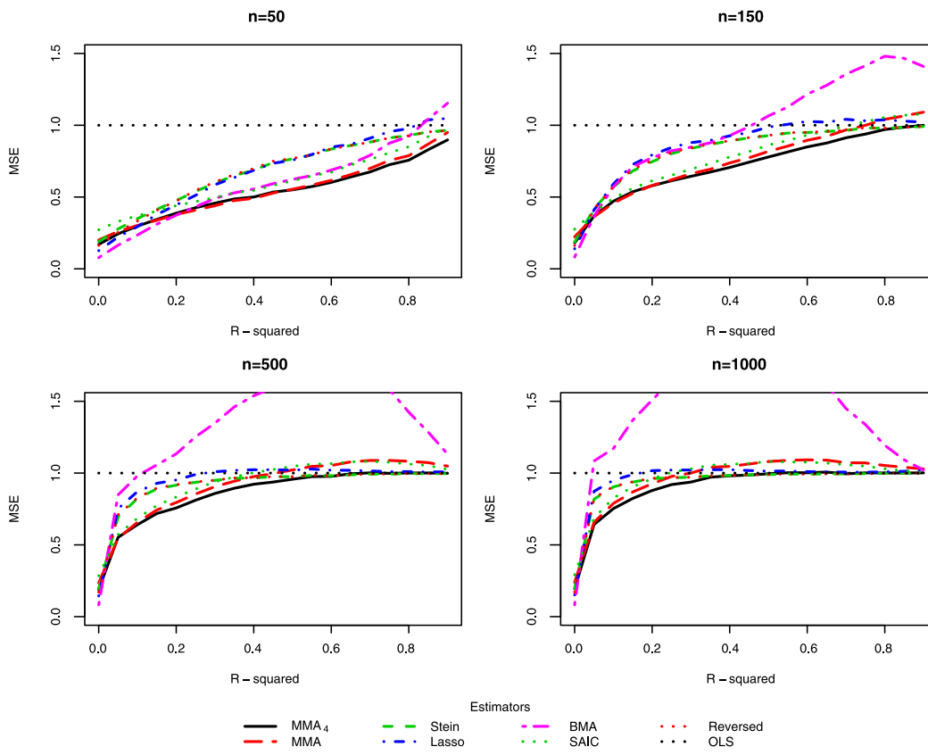
FIGURE 10. Model 3: \alpha = 1 .
