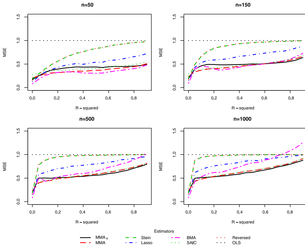
FIGURE 11. Model 3: \alpha = 2 .
