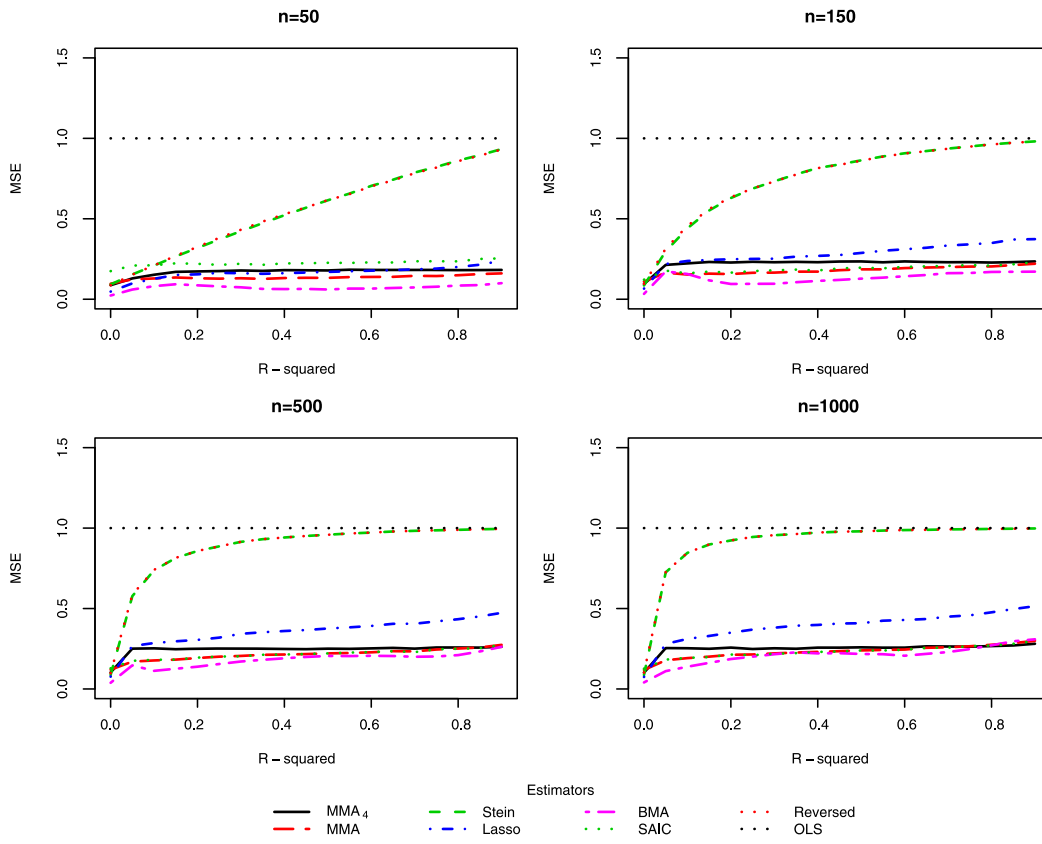
FIGURE 20. Model 5: \alpha = 3 .
