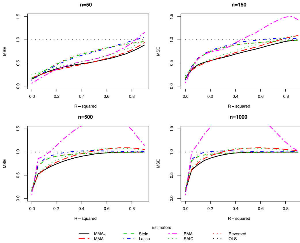
FIGURE 2. Model 1: \alpha = 1 .
