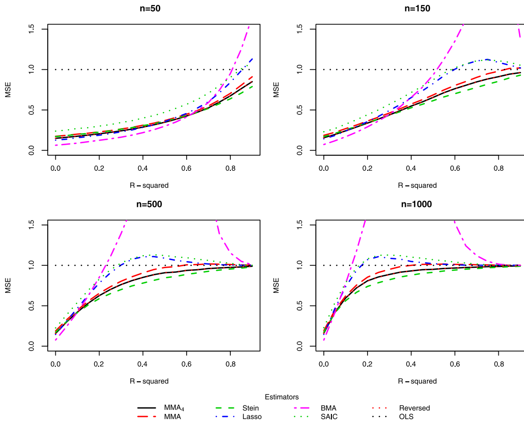
FIGURE 1. Model 1: \alpha = 0 .
