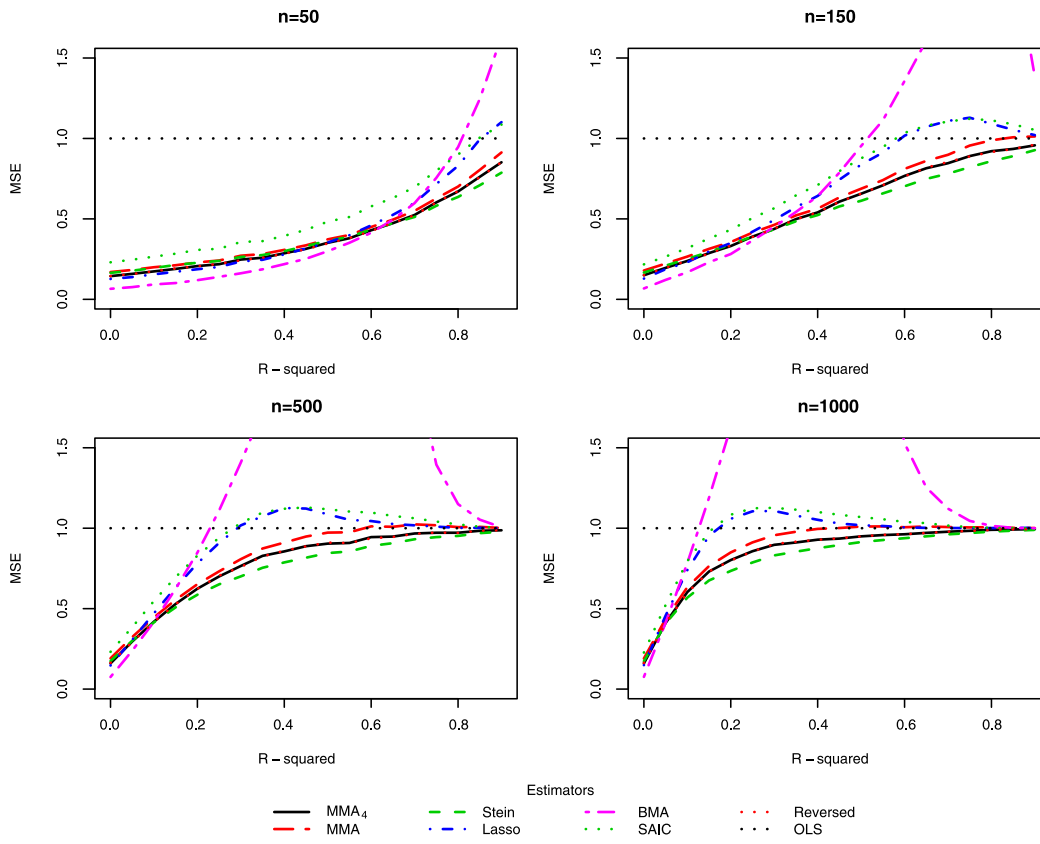
FIGURE 5. Model 2: \alpha = 0 .
