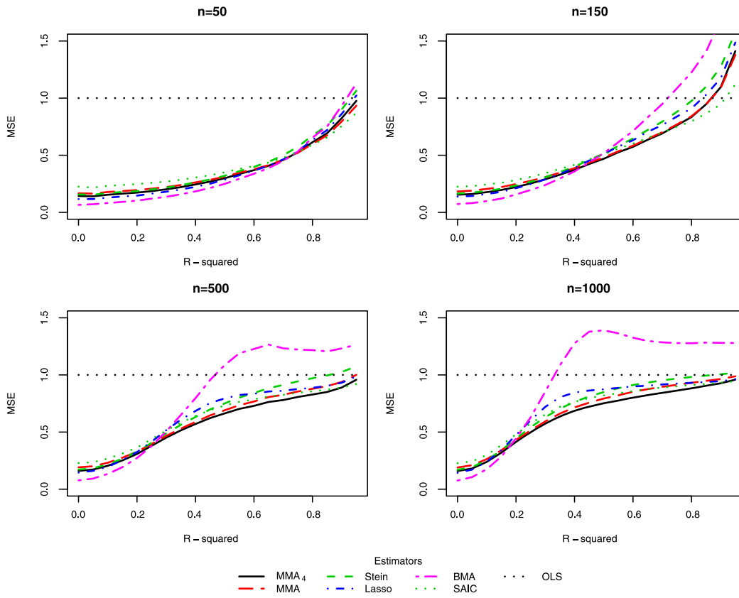
FIGURE 21. Model 6: Autoregression.
