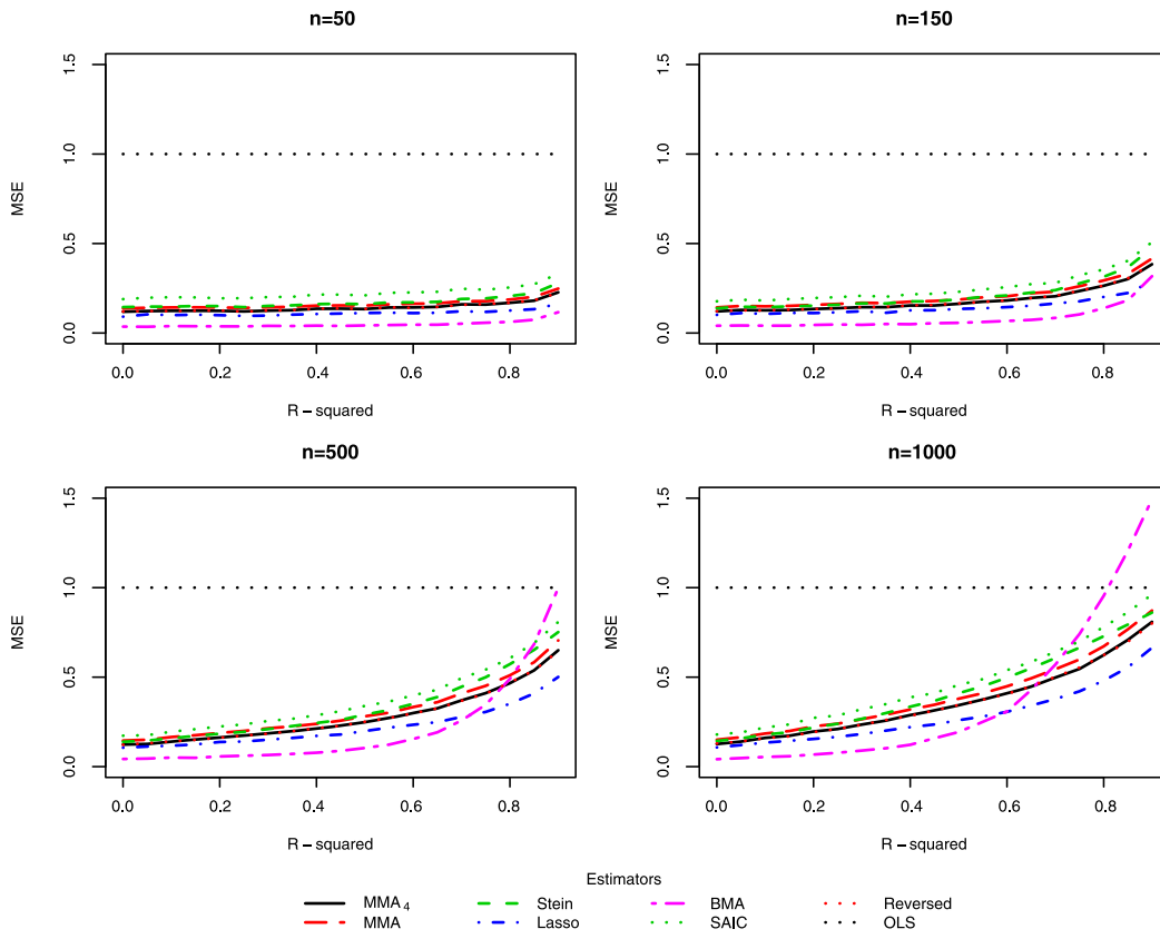
FIGURE 13. Model 4: \alpha = 0 .
