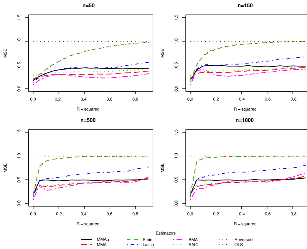
FIGURE 12. Model 3: \alpha = 3 .
