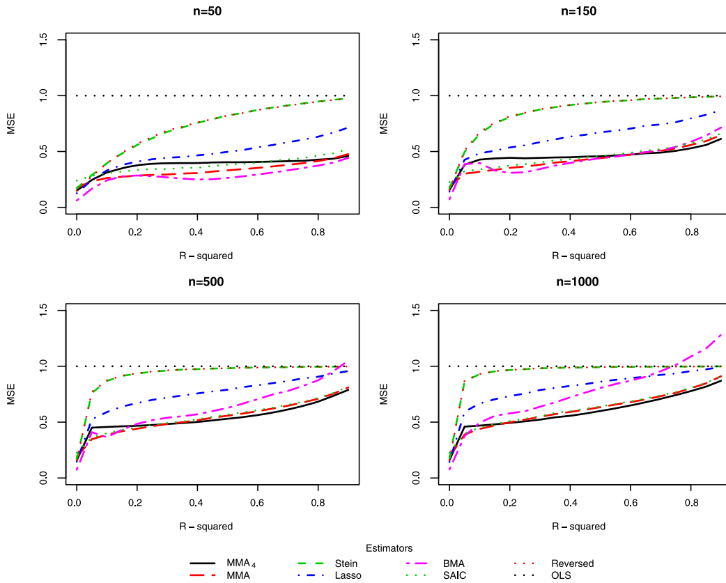
FIGURE 3. Model 1: \alpha = 2 .
