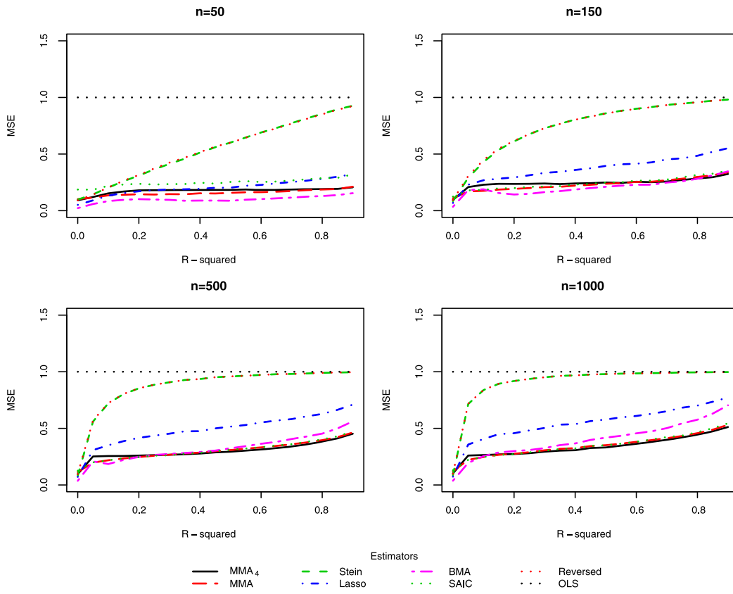
FIGURE 19. Model 5: \alpha = 2 .
