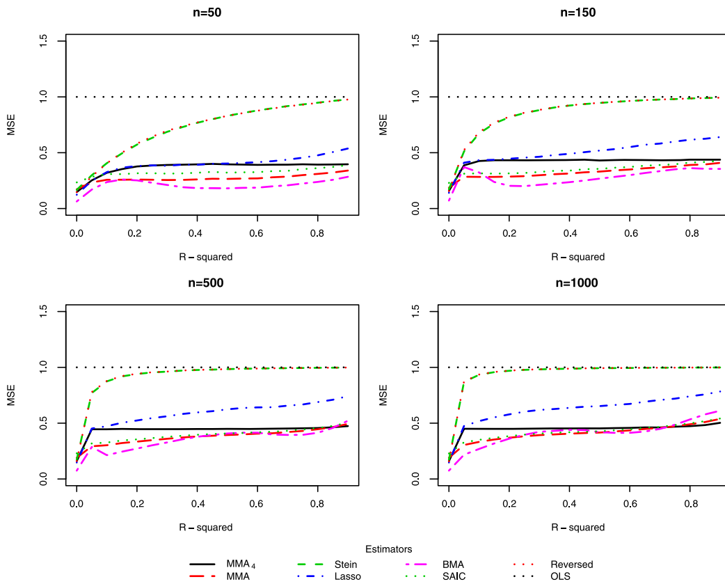
FIGURE 4. Model 1: \alpha = 3 .
