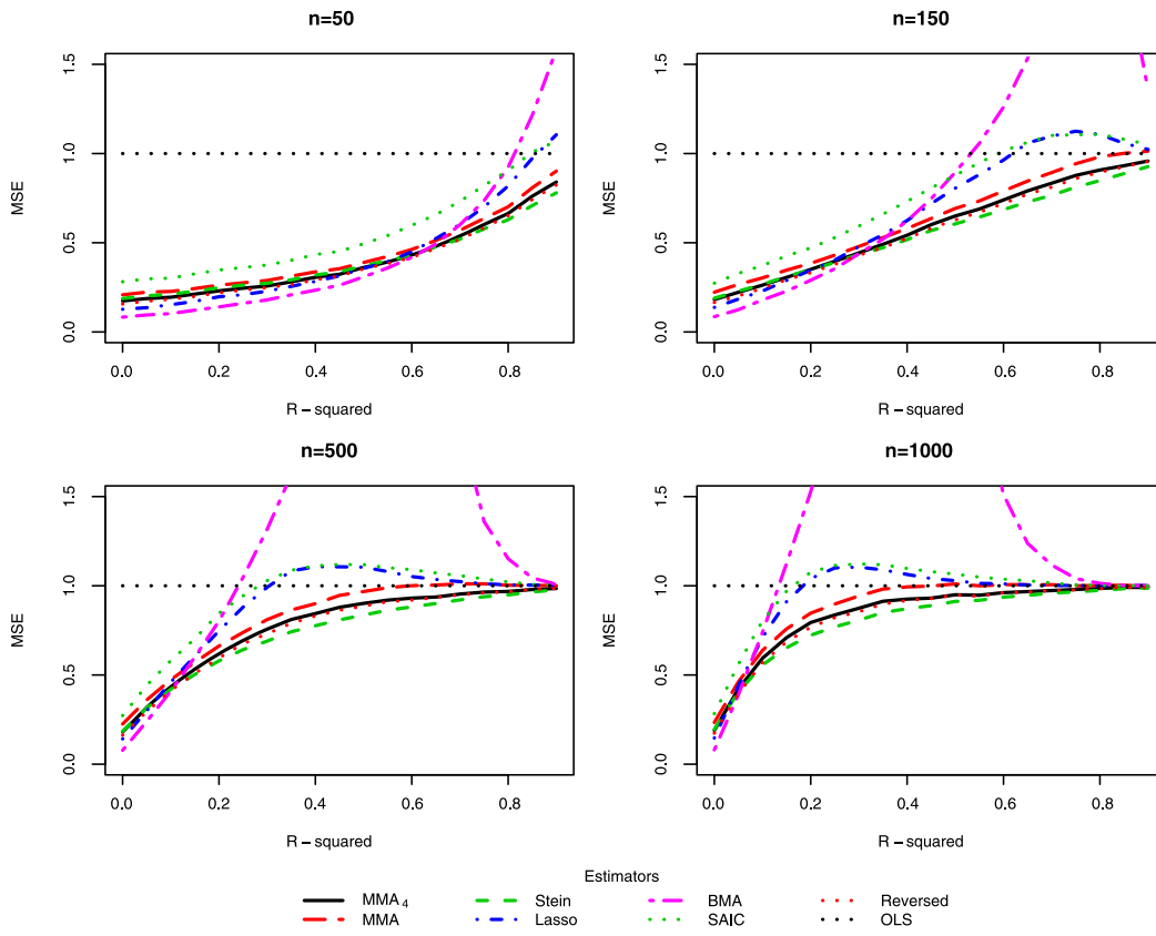
FIGURE 9. Model 3: \alpha = 0 .
