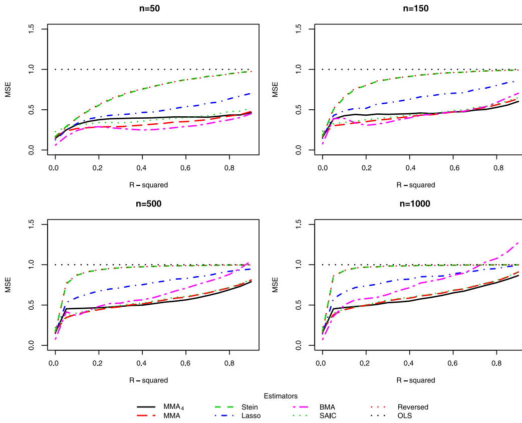
FIGURE 7. Model 2: \alpha = 2 .
