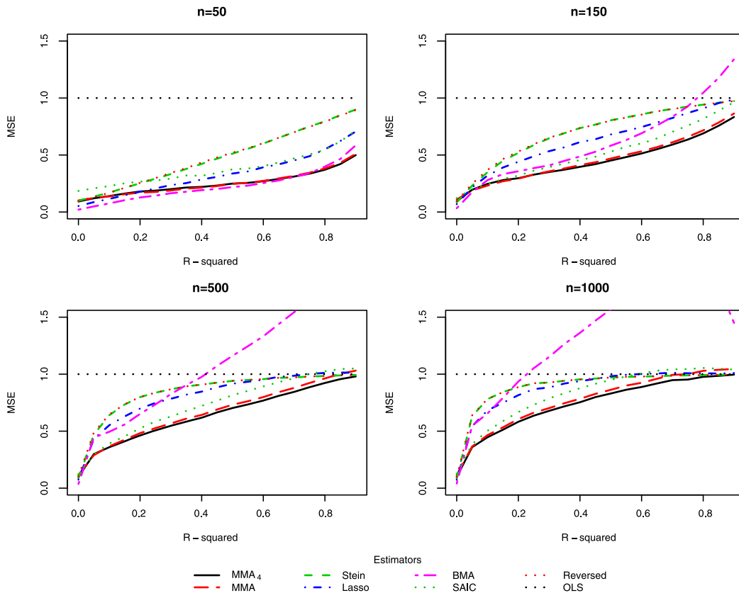
FIGURE 18. Model 5: \alpha = 1 .
