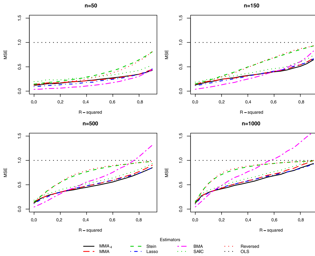
FIGURE 14. Model 4: \alpha = 1 .
