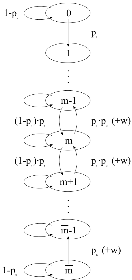
Figure 2: The Markov chain resulting from the optimal policy.
