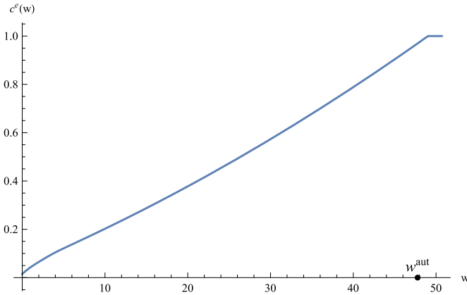
FIGURE 6. Consumption of the agent when employed as a function of w \in \mathcal{W} . The figure shows the graph of the consumption of the employed agent as a function of w —the expected discounted utility promised to the agent. The autarky utility level is w^{\text{aut}} = 47.7736 .
