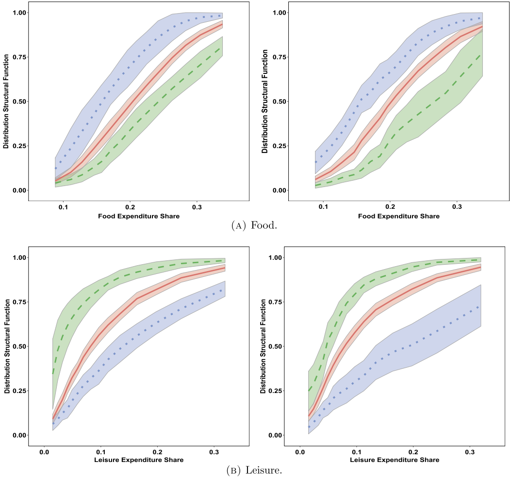
FIGURE 3. DSE DSF at X = \widehat{Q}_X(0.1) (dashed), X = \widehat{Q}_X(0.5) (solid), X = \widehat{Q}_X(0.9) (dotted). Quantile (left) and distribution regression (right).
