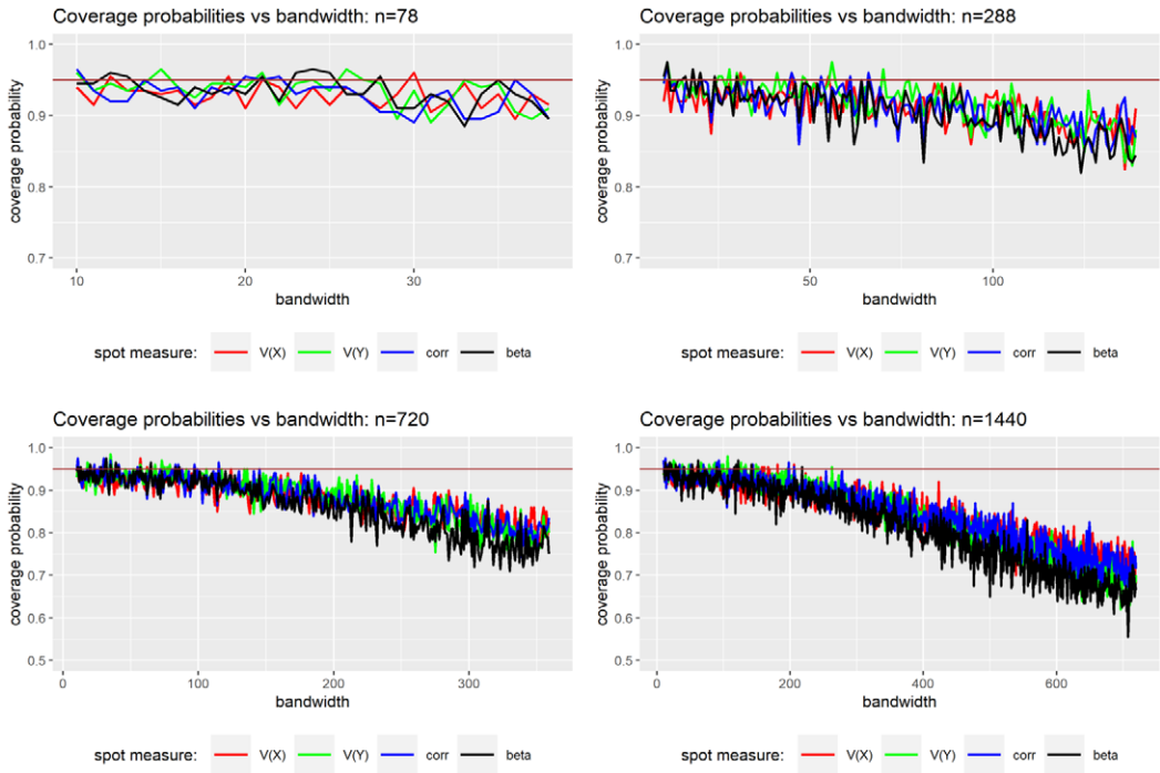
FIGURE 2. Coverage probability and the bandwidth. This picture examines the robustness of the coverage for the new Laplace transform-based spot measure estimators to the bandwidth parameter, k_n , using local Gaussian bootstrap inference. Specifically, the upper left depict a scenario where n = 78 and k_n \in [10, 39) ; upper right where n = 288 and k_n \in [10, 144) ; lower left where n = 720 and k_n \in [10, 360) ; and lower right where n = 1440 and k_n \in [10, 720) . The spot measures are estimated using parameters u_{\min} = 1/100 , u_{\max} = 1/5 with step length 1/100 and a uniform kernel. Moreover, they are localized around \tau = 1/2 in all cases. The nominal level of the coverage is 95%. The simulations are implemented with 10,000 replications, each of which uses 999 bootstrap draws.
