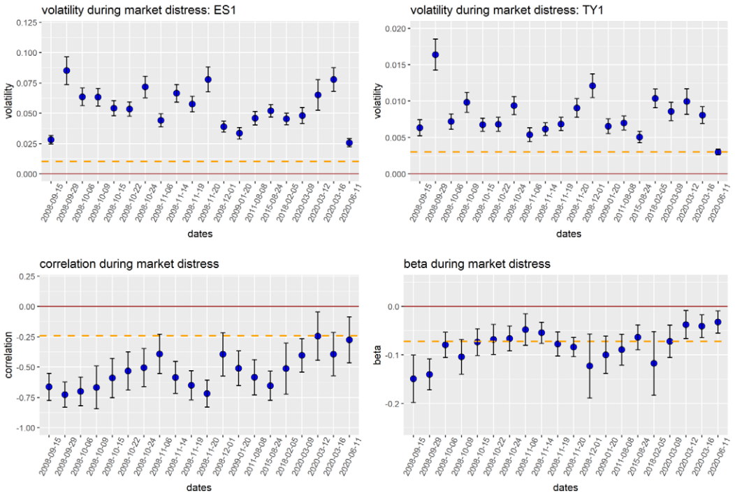
FIGURE 3. Risk measures during market distress. This picture displays end-of-day spot volatility, correlation, and market beta estimates together with associated 95% confidence intervals based on the local Gaussian bootstrap for the 20 days with the worst daily return on S&P 500 futures contracts (ES1). Moreover, the dashed orange line provide the average spot measure estimate over the full sample from January 2005 through December 2020. The estimates of the spot measures are implemented as described in Table 4.
